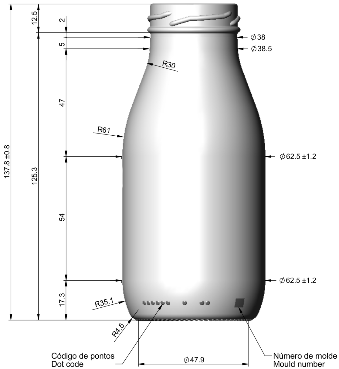
Vista Frontal Front View
